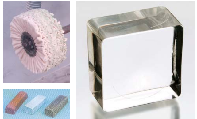
Polishing with felt belt or disc turret fitted with cotton or flanel buffer and polishing agent
