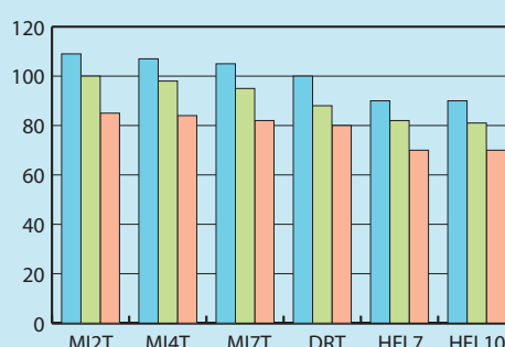
Figure 2b: Thermal properties Altuglas® high impact grades
