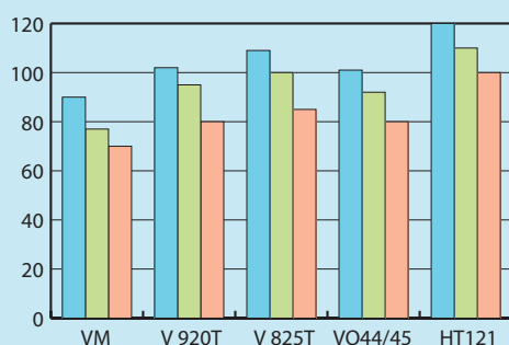
Figure 2a: Thermal properties Altuglas® standard grades
