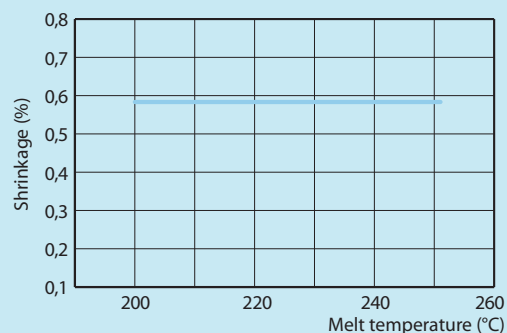
Shrinkage vs melt temperature
