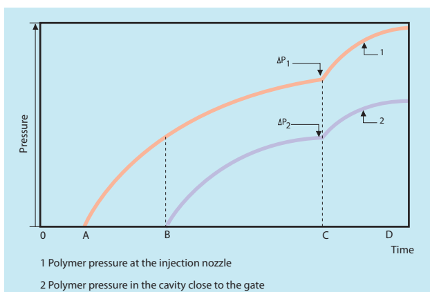
Variation in pressure versus time
