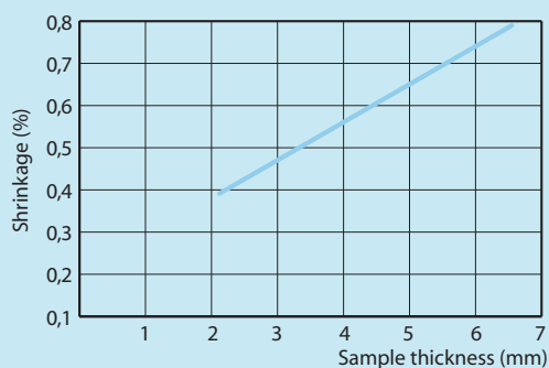
Shrinkage vs thickness
