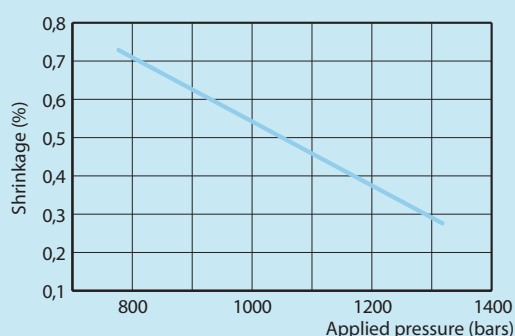
Shrinkage vs applied pressure
